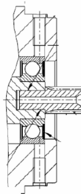
Motor Shaft with fitted Pinion
